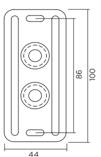
TRAIN 2.0 - wall base dimensions
