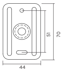
TRAIN 2.0 - wall base dimensions
